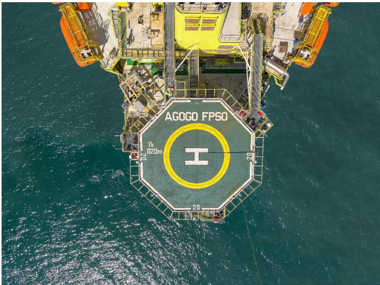
Top view of Agogo FPSO helideck
